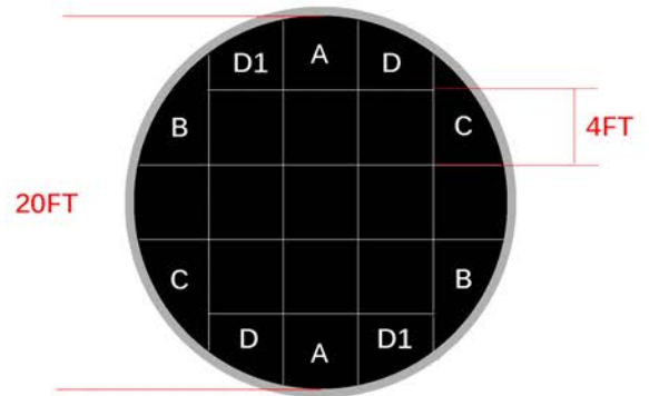
Wooden dance floor Diameter 20ft
